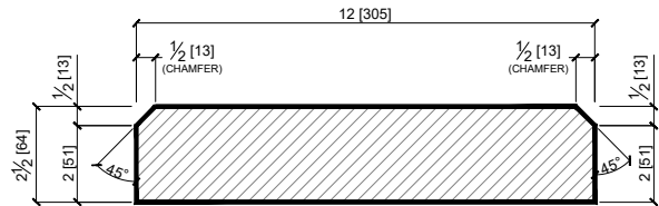
POOL COPING PROFILE - PC06 (W/ DOUBLE 45° CHAMFER - N.T.S)
