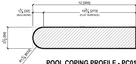
POOL COPING PROFILE - PC01 (W/ BULLNOSE - N.T.S)
