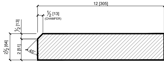
POOL COPING PROFILE - PC05 (W/ 45° CHAMFER - N.T.S)
