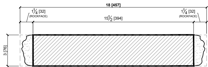
POOL COPING PROFILE - PC08 (W/ DOUBLE ROCK FACE - N.T.S)
