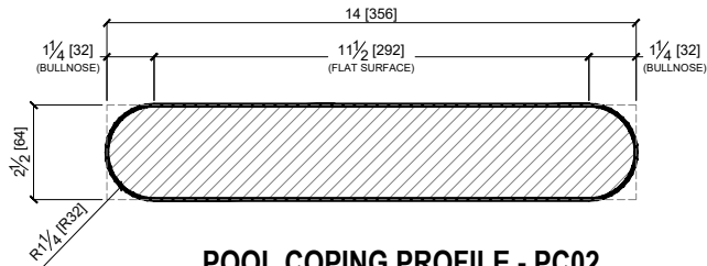
POOL COPING PROFILE - PC02 (W/ DOUBLE BULLNOSE - N.T.S)
