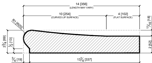
POOL COPING PROFILE - PC04 (W/ CURVED LIP - N.T.S)
