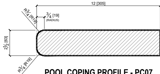
POOL COPING PROFILE - PC07 (W/ RADIUS EDGES - N.T.S)
